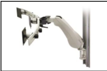
HD Triple-Monitor Arm, grey, shown with Vertical Mount on Wall Track. Pivots on crossbar accommodate monitors up to 20" (508 mm) wide. This multiple-monitor mounting system utilizes Ergotron's patented Paraview Technology.
