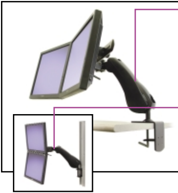
HD Dual-Monitor Arm shown with Desk Clamp Mount. Crossbar tilts monitors up 25° and down 10° using small lever behind monitors. Maximum monitor width is 23-1/4" (590 mm).
